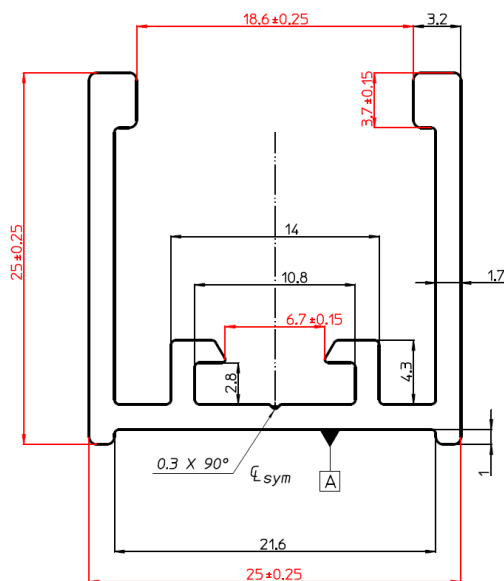
HK3106: U-profile
