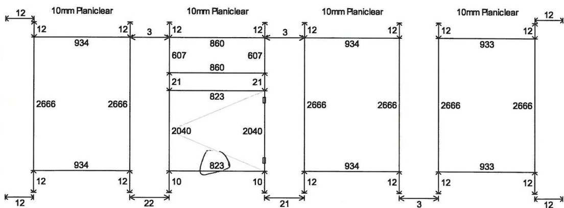
Size details of glass elements and spacing used in test wall.
