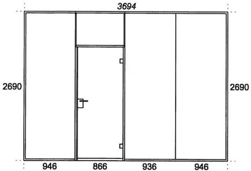
Glass partition test wall and door in test opening including mounting profiles.
